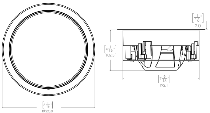
6.5” Flush Mount Kit Dimensions
