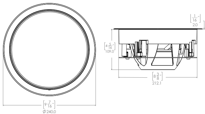
7.7” Flush Mount Kit Dimensions
